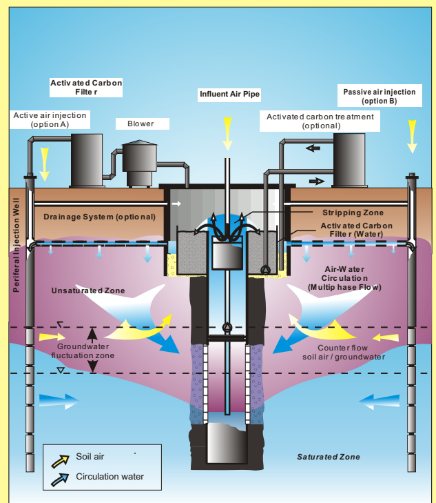
IEG Soil Circular Flushing™ System for biological-physical remediation of the unsaturated zone (IEG SZB™ Process)
